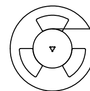
EMBOSSED CARRIER TAPE WITH DIMENSIONS
