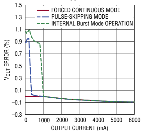
Load Regulation ( V_{IN} = 3.3V , V_{OUT} = 1.8V )
