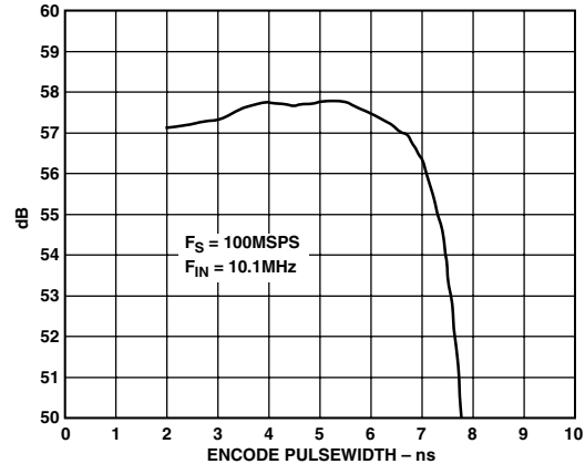
Figure 15. SNR vs. Clock Pulse Width ( t_{EH} )
