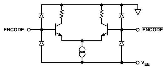
Figure 4. Equivalent Encode Input Circuit
