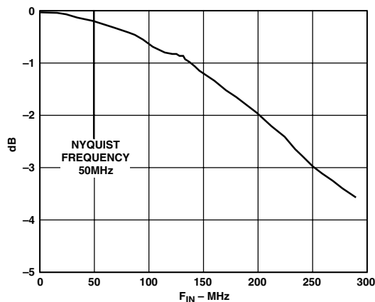
Figure 16. Frequency Response
