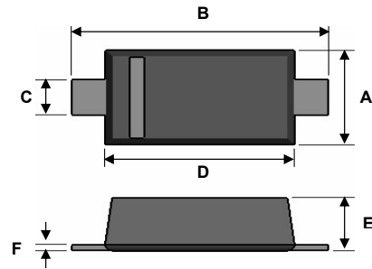
SOD-523F
