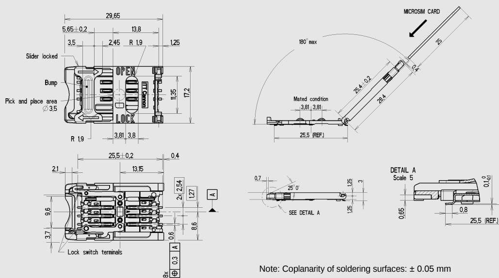
Hinged Cover CCM03-3514 (6 contacts - with switch on metal lock)
