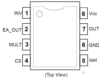
Figure 2. Pin Configuration
