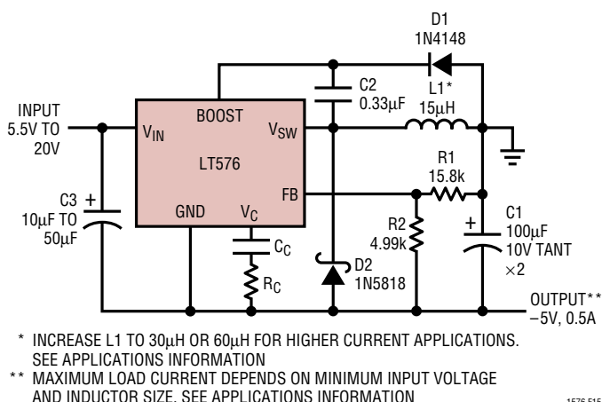
Figure 15. Positive-to-Negative Converter
