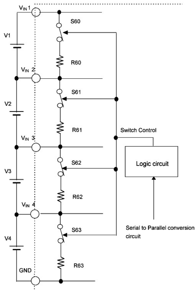
Figure 11. Conditioning Circuit
