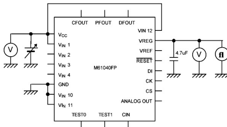
Circuit 3
