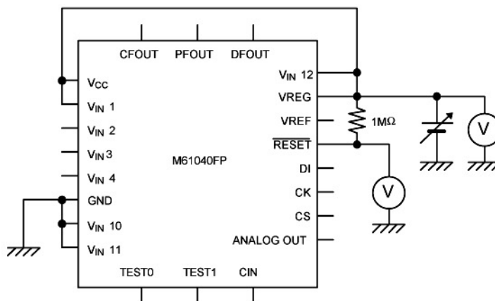
Circuit 2
