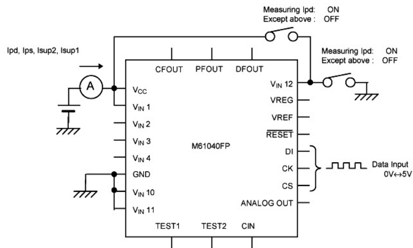
Circuit 7
