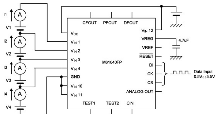
Circuit 6
