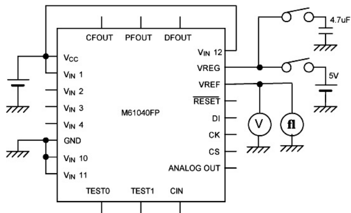
Circuit 4
