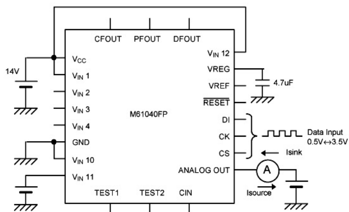
Circuit 9
