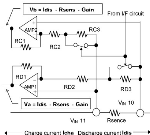
Figure 7. Charge/Discharge current detection
