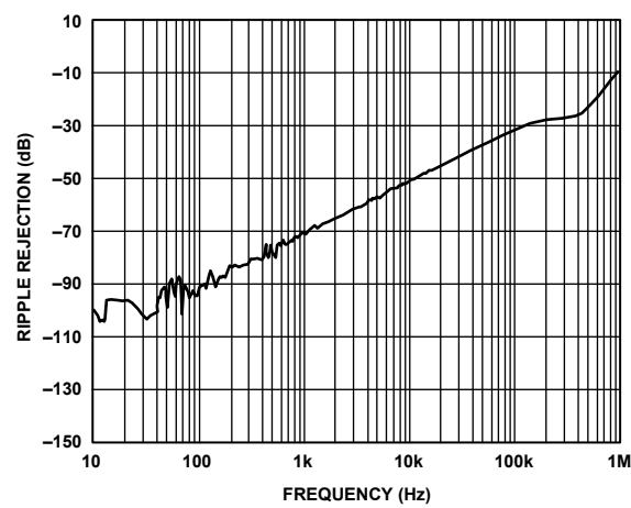
Figure 28. Ripple Rejection Ratio
