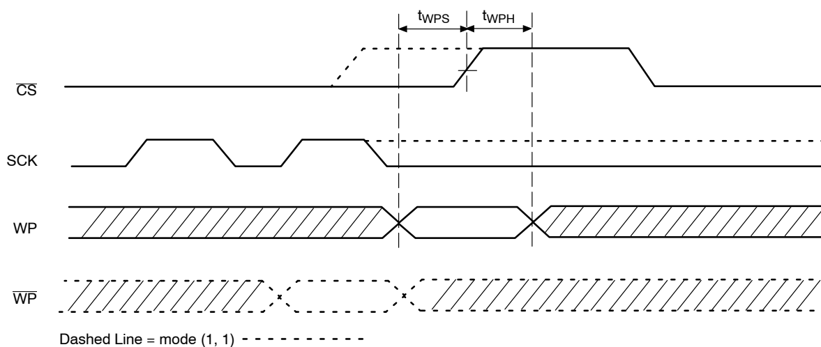
Figure 8. \overline{WP} Timing
