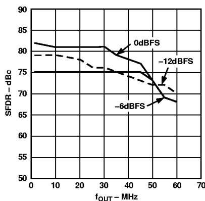
Figure 11. "In-Band" SFDR vs. f_{OUT} @ f_{DATA} = 150 MSPS
