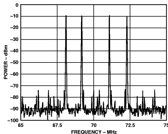
Figure 53. Spectral Plot of Four Carriers at 70 MHz IF with f_{\text{DATA}} = 52 MSPS, PLLVDD = 0
