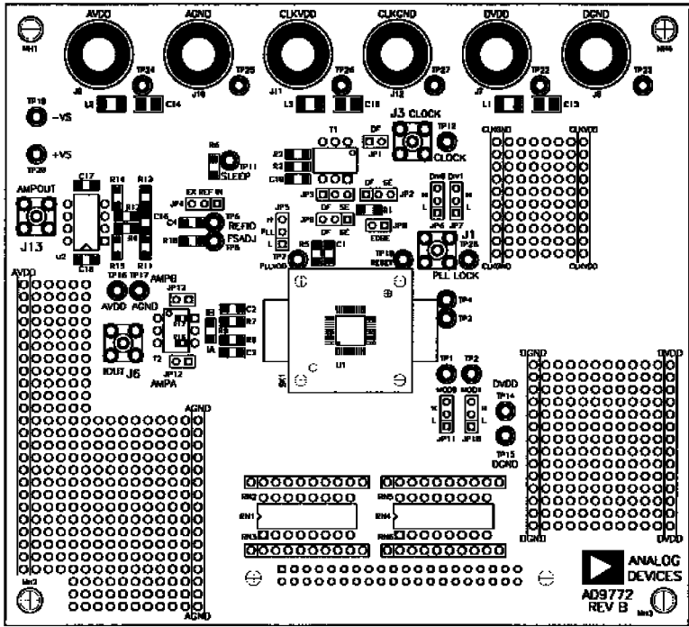
Figure 56. Silkscreen Layer-Top
