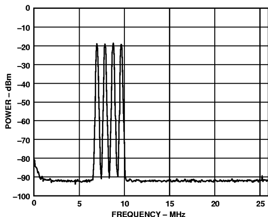
Figure 49. Spectral Plot of AD9772 Reconstructing Four GSM Modulated Carriers @ f_{\text{DATA}} = 52 \text{ MSPS} , \text{PLLVD} = 0
