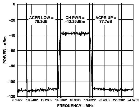
Figure 50. AD9772 Achieves 78 dB ACPR Performance Reconstructing a "WCDMA-Like" Test Vector with f_{\text{DATA}} = 65.536 \text{ MSPS} and \text{PLLVD} = 0
