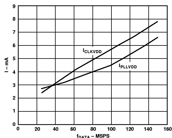
Figure 40. I_{PLLVD} and I_{CLKVDD} vs. f_{DATA}
