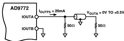
Figure 44. 0 V to +0.5 V Unbuffered Voltage Output
