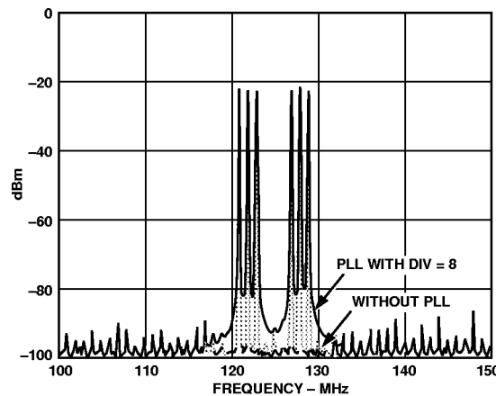
Figure 28. Direct IF Mode Reveals Phase Noise Degradation With and Without PLL Clock Multiplier (IF = 125 MHz and f_{\text{DATA}} = 100 MSPS)
