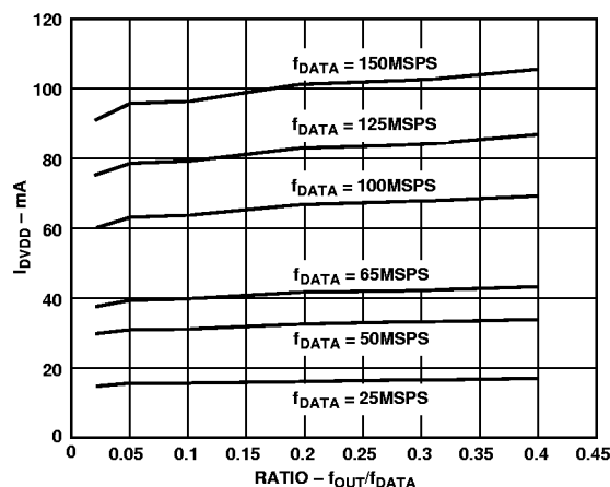
Figure 39. I_{DVDD} vs. Ratio @ DVDD = 3\text{ V}
