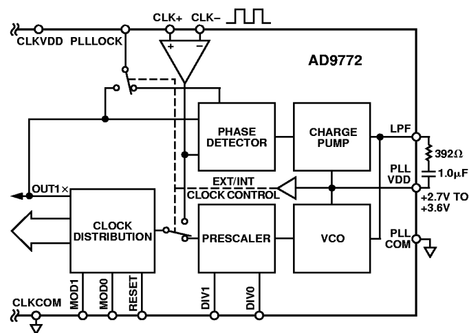
Figure 26. Clock Multiplier with PLL Clock Multiplier Enabled
