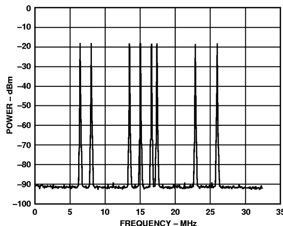
Figure 48. Spectral Plot of AD9772 Reconstructing Eight IS-136 Modulated Carriers @ f_{DATA} = 64.54 MSPS, PLLVDD = 0
