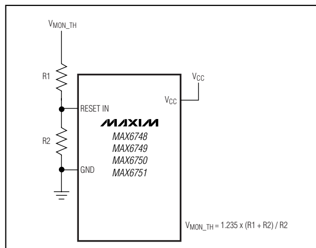
Figure 2. Calculating the Monitored Threshold Voltage ( V_{\text{MON\_TH}} )
