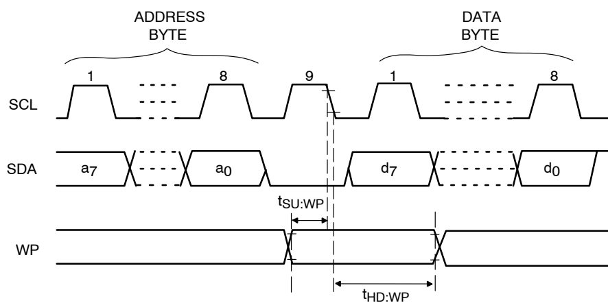
Figure 9. WP Timing
