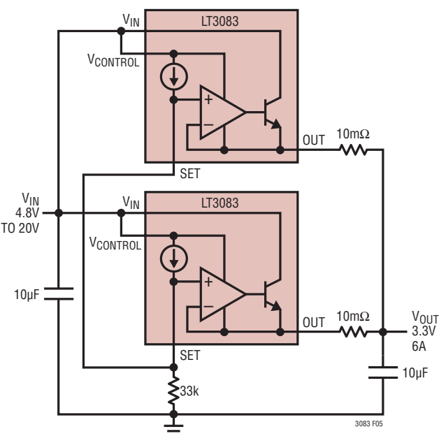
Figure 5. Parallel Devices
