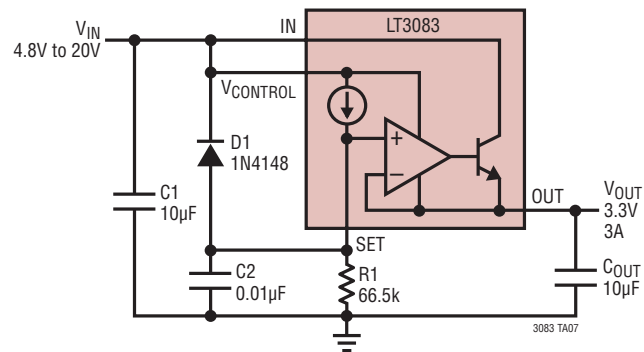
Adding Soft-Start
