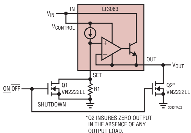
Adding Shutdown
