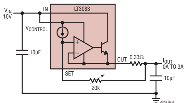
Current Source
