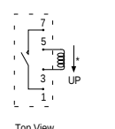
MVS4/MSS4 Pinout
