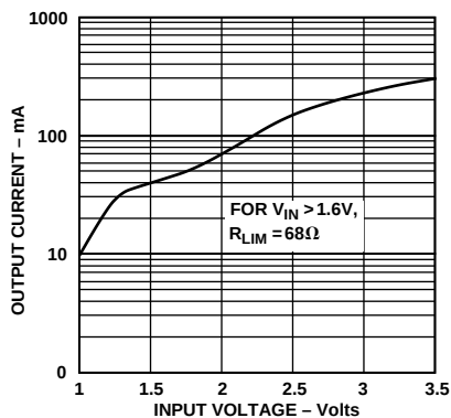
Figure 5. Guaranteed Minimum Output Current at V_{OUT} = 5V vs. Input Voltage
