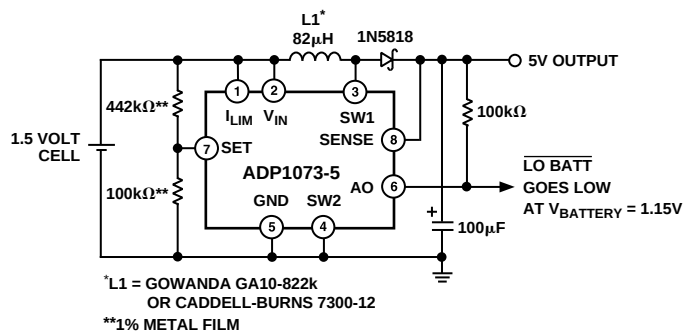
Figure 34. 1.5 V to 5 V Step-Up Converter with Low Battery Detector
