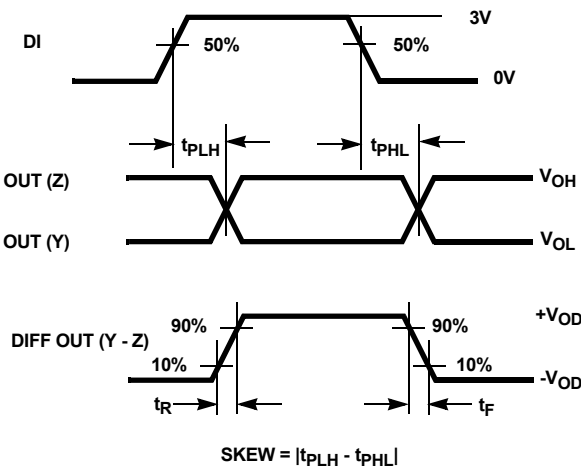
FIGURE 6B. MEASUREMENT POINTS
