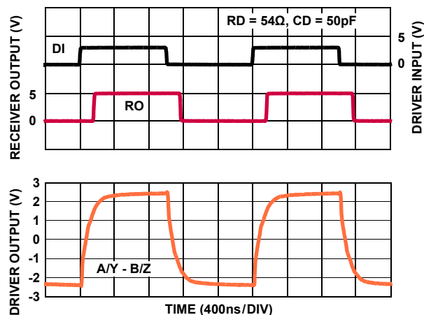
FIGURE 21. DRIVER AND RECEIVER WAVEFORMS
