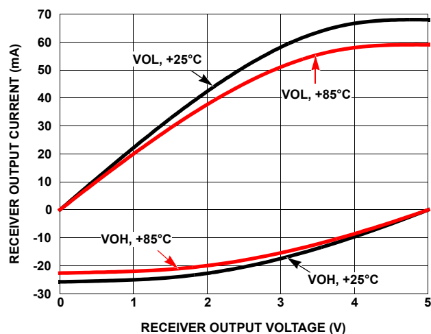
FIGURE 16. RECEIVER OUTPUT CURRENT vs RECEIVER OUTPUT VOLTAGE
