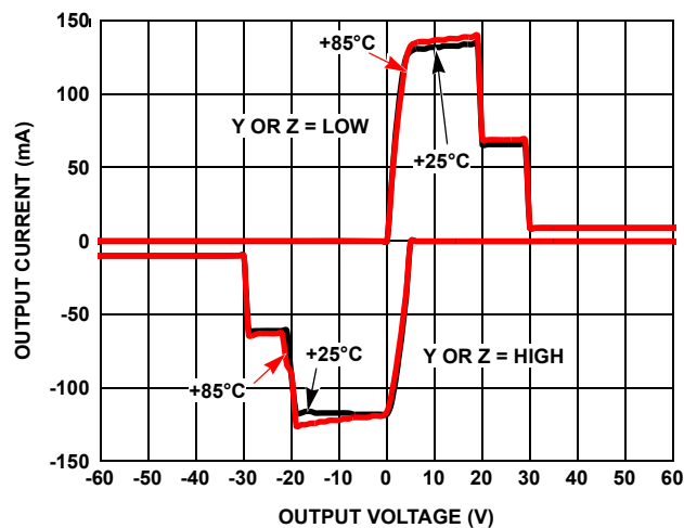
FIGURE 15. DRIVER OUTPUT CURRENT vs SHORT-CIRCUIT VOLTAGE
