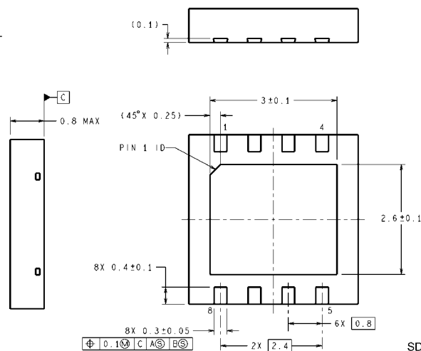
8-Lead LLP Package NS Package Number SDC08A
