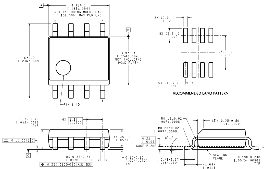
8-Lead SO-8 Package NS Package Number M08A
