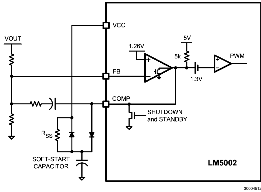
FIGURE 5. Soft-Start
