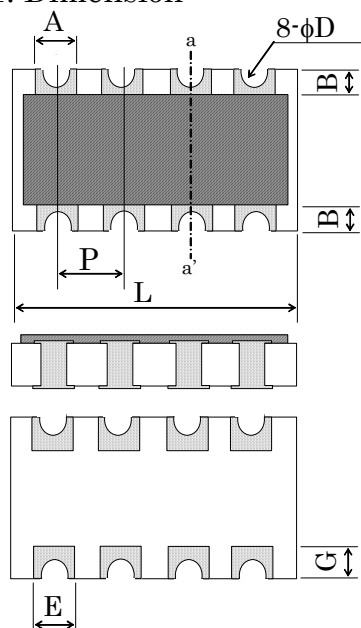
a-a' sectional plan
