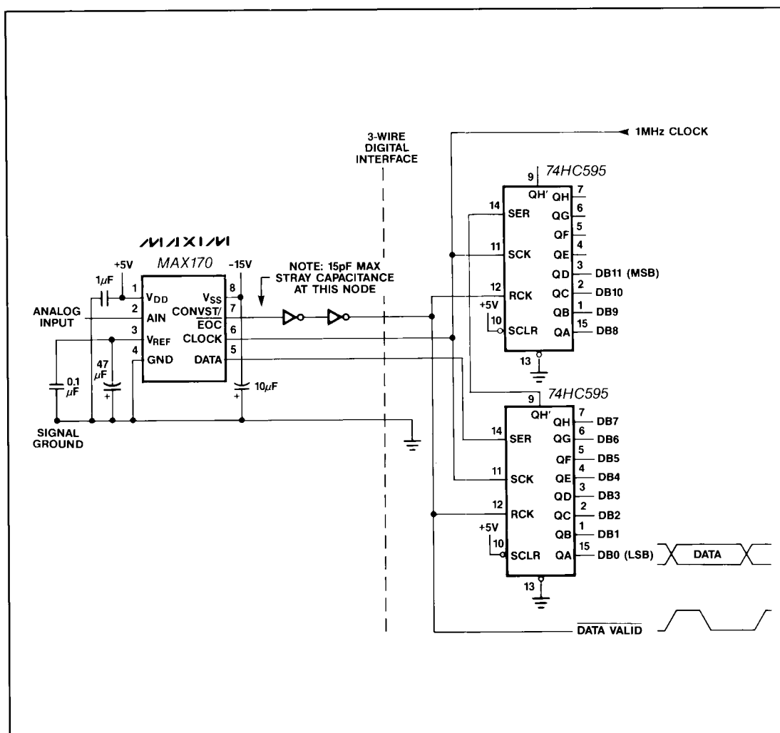
Figure 15. Self-Start Mode
