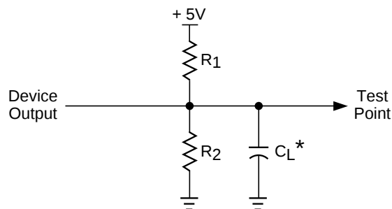
Figure 2. Test Load
