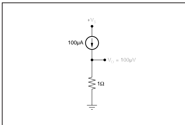
FIGURE 21. Low-Voltage Reference.
