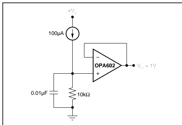
FIGURE 22. Voltage Reference.
