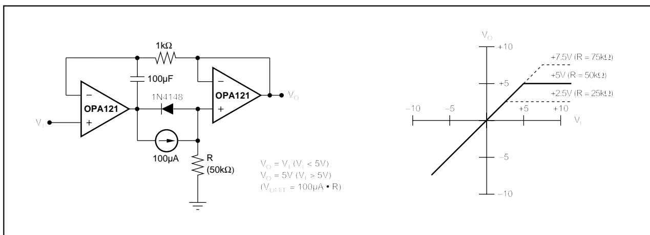
FIGURE 24. Limiting Circuit.
