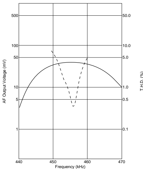
CDBLA/CDBLB455KCAY42-B0
