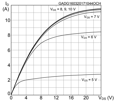
Figure 7. Output characteristics
