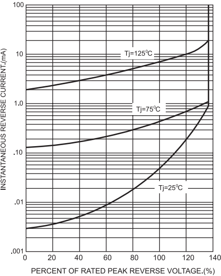
FIG.3-TYPICAL REVERSE CHARACTERISTICS
