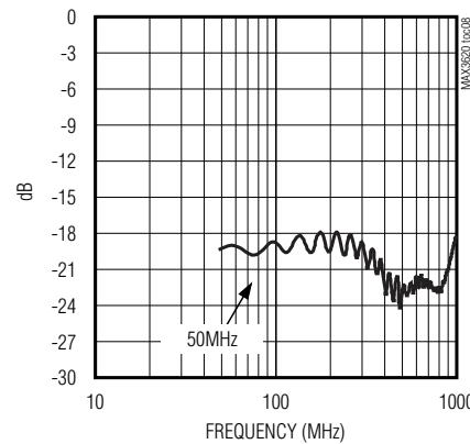
MAX3620D S11
