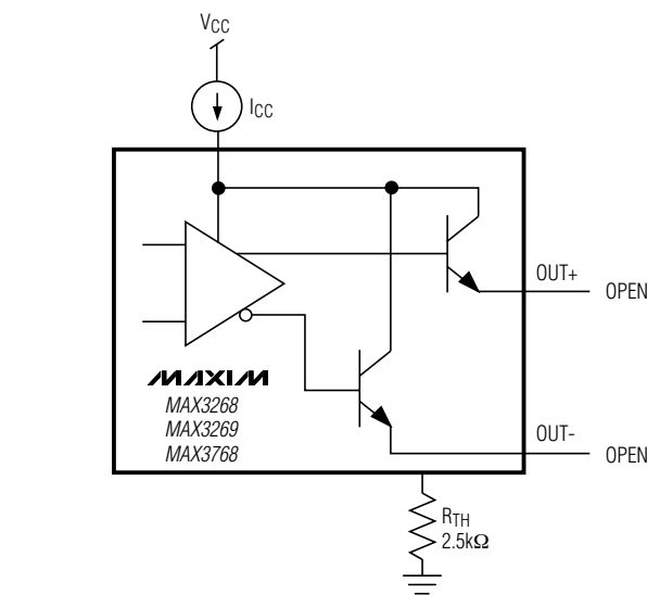
(b) PECL SUPPLY CURRENT ( I_{CC} )
