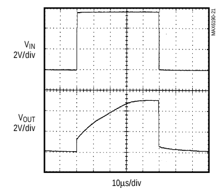
MAX6195 TURN-ON TRANSIENT
