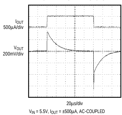
MAX6195 LOAD-TRANSIENT RESPONSE
