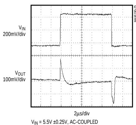
MAX6195 LINE-TRANSIENT RESPONSE
