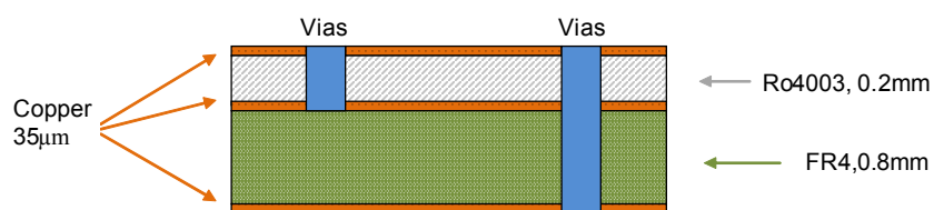
BGA824N6_application_board_sideview.vsd
