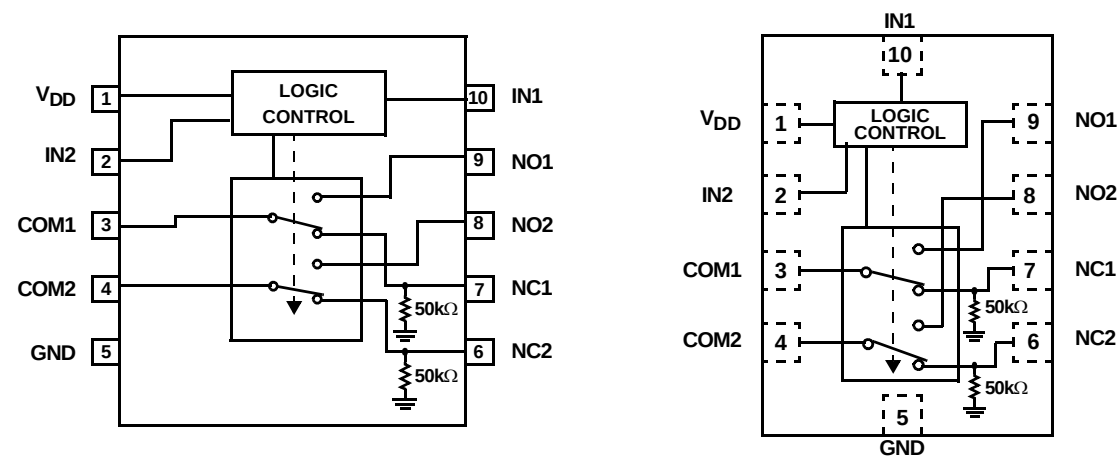
ISL54402 (TDFN, \mu TQFN) TOP VIEW
