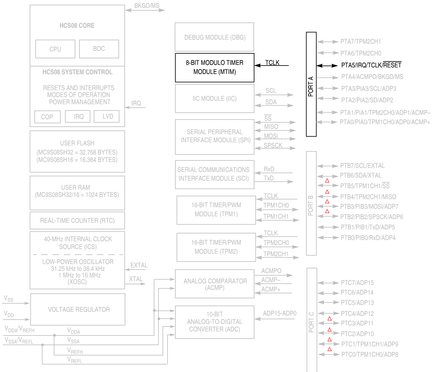
Figure 12-1. MC9S08SH32 Series Block Diagram Highlighting MTIM Block and Pins
