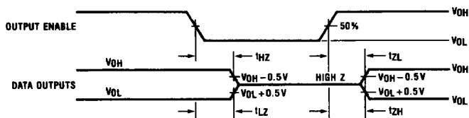
FIGURE 17. TRI-STATE Test
