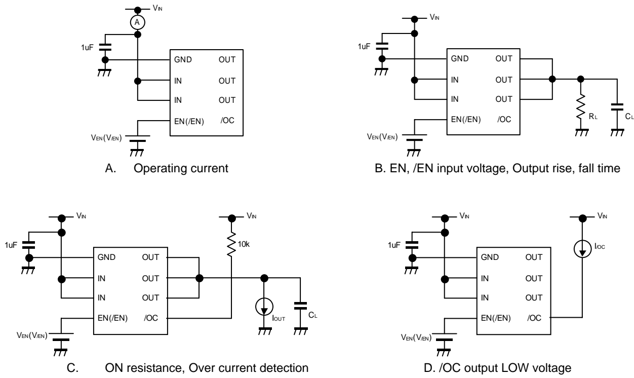
Figure 1. Measurement circuit
