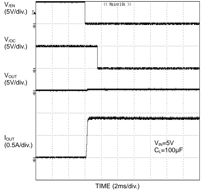
Figure 31. Over current response Enable to shortcircuit (BD2041AFJ)
