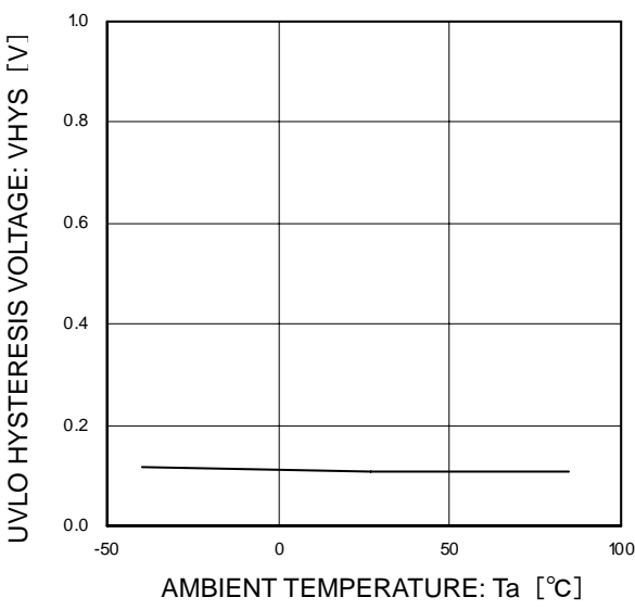
Figure 25. UVLO hysteresis voltage
