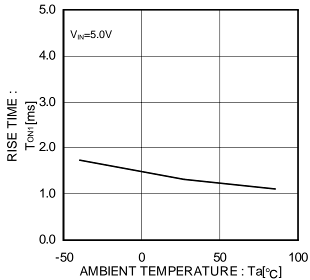
Figure 17. Output rise time
