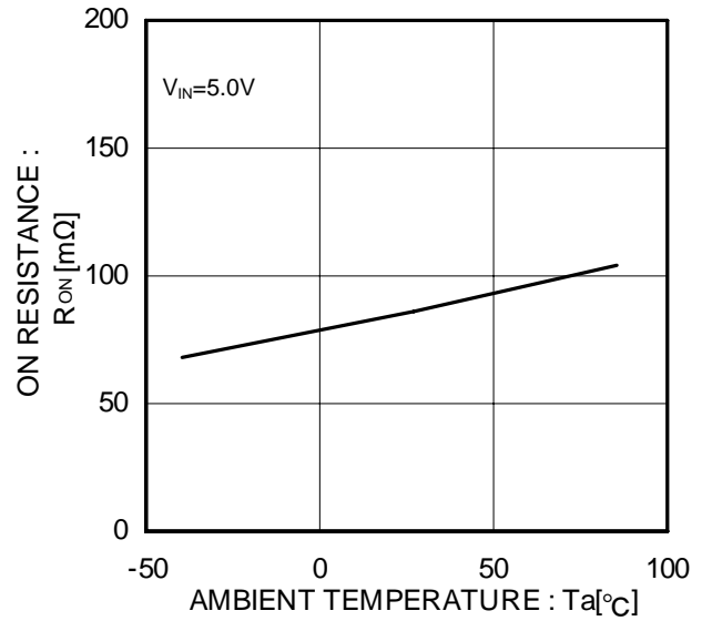
Figure 13. ON resistance
