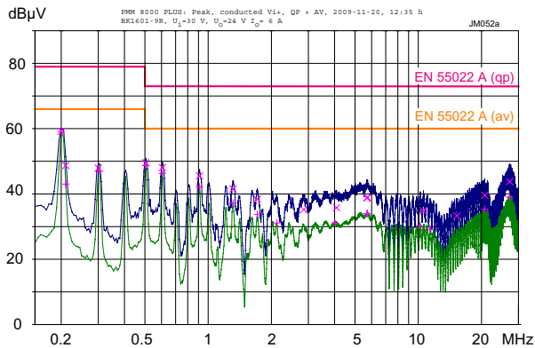
Fig. 22a Conducted emissions (peak/quasipeak and average) at the phase input according to EN 55011/22, measured at V_{inom} and I_{onm} (BK1601-9R). The neutral line performs quite similar.
