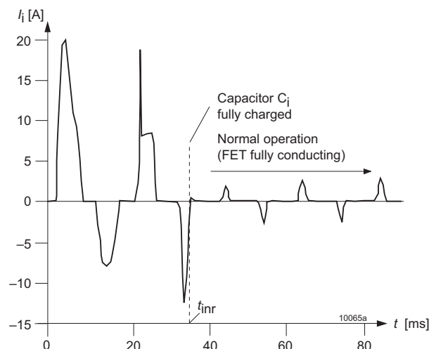
Fig. 32 Inrush current for LK models with option E (AC supply) V_i = 230 \text{ VAC} , f_i = 50 \text{ Hz} , P_o = P_{o \text{ nom}}
