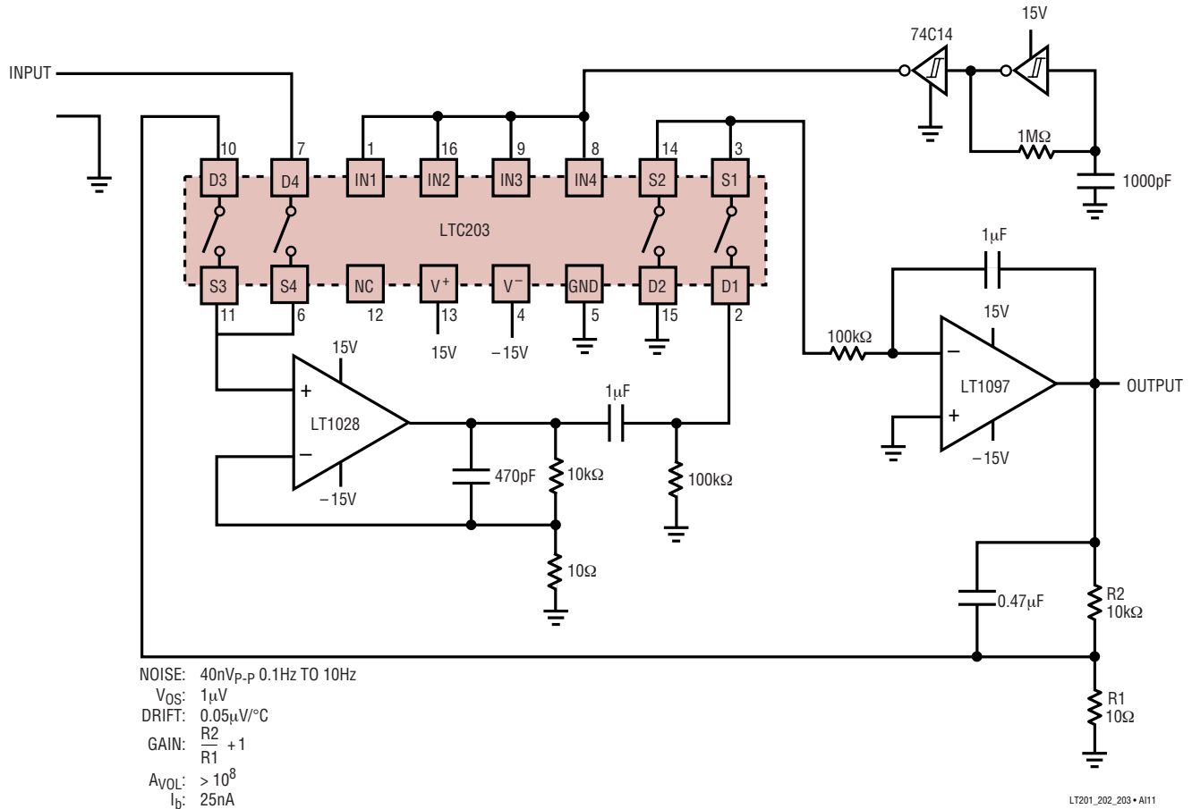
Ultra Low Noise, Low Drift Chopper Amplifier
