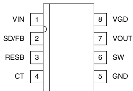
TSSOP-8 (TOP VIEW) PW Package
