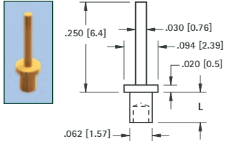
.030 (.76) PIN - SWAGE MOUNT
