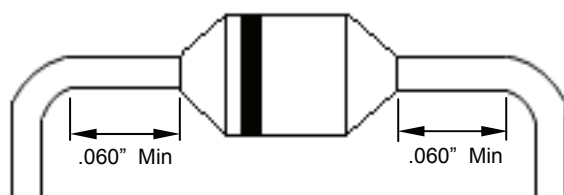
Case Style 401 & 402 Minimum Bend Distance
