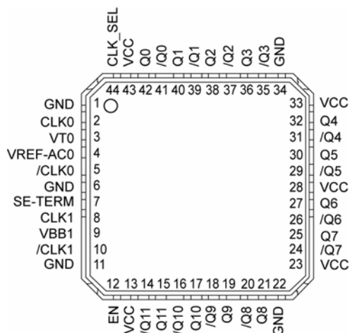
44-Pin MLF TM (MLF-44)
