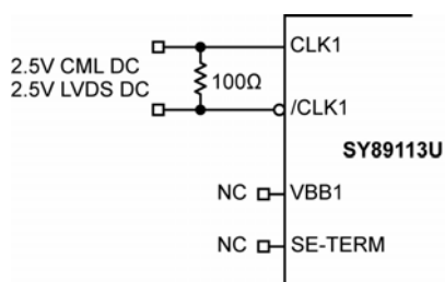
Figure 4a. CML, LVDS Interface (DC-Coupled)
