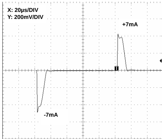
FIGURE 27. LOAD TRANSIENT RESPONSE, 0.001µF LOAD CAPACITANCE
