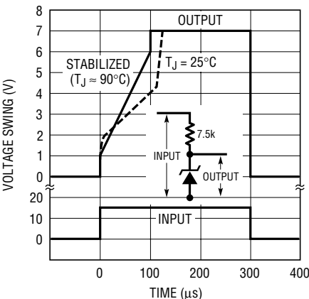
Response Time
