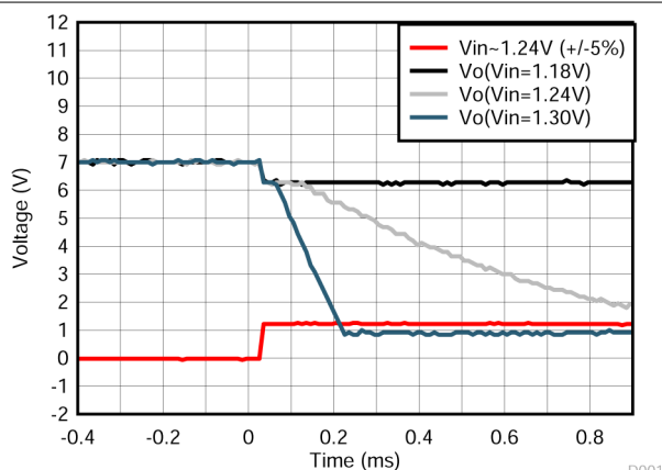
Figure 8-3. Output Response with Small Overdrive Voltages
