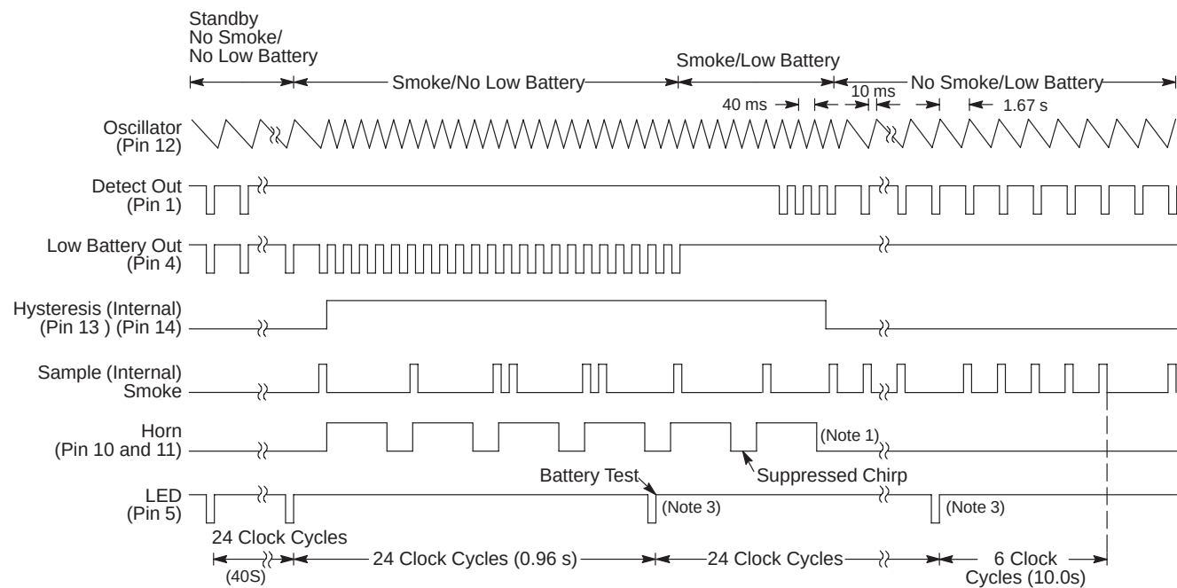
Figure 6. Timing Diagram
