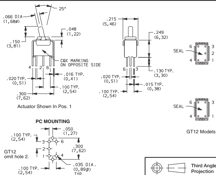
PART NUMBER SWITCH FUNCTION POS.1 POS. 2 POS. 3 GT11MV3BE GT13MV3BE ON ON NONE OFF ON ON Conn. Terms. 2-3 OPEN 2-1 Schematic SPDT Note: Pins 4 and 6 not connected GT12MV3BE OFF NONE ON Conn. Terms. OPEN N/A 3-1 Schematic SPST Note: Pins 4 and 6 not connected
