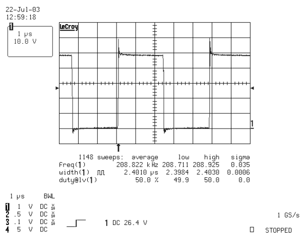
FIGURE 15. FET DRAIN-SOURCE VOLTAGE
