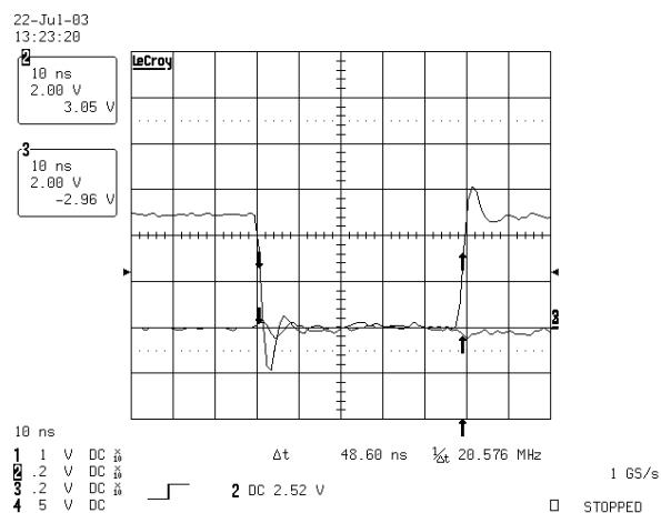
FIGURE 17. OUTA TO OUTB TRANSITION
