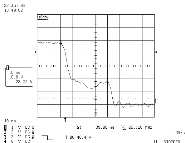
FIGURE 16. FET D-S VOLTAGE NEAR-ZVS TRANSITION
