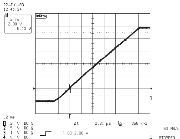
FIGURE 13. OUTPUT SOFT-START
