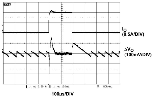
FIGURE 19. LOAD TRANSIENT RESPONSE (22mA to 1A)
