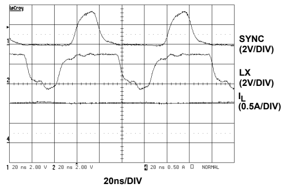
FIGURE 18. EXTERNAL SYNCHRONIZATION TO 12MHz
