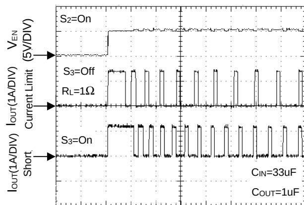
Thermal Shutdown Response ⑤
