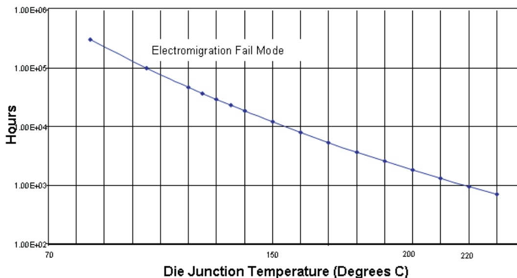
Figure 6-1. SM470R1B1M-HT Life Expectancy Curve (HFQ/HKP Package)
