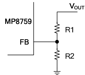
Figure 7: Feedback Network
