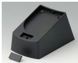
A9176139 Station XS ABS (UL 94 HB) black RAL 9005
